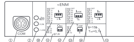
Diagram 10. NM8N-400, 630 ENM 3P (Motor protection ) Controller interface
