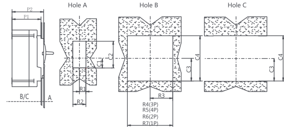
Diagram 6. NM8N(DC, SD)-125 ~ 1600 front opening hole size
